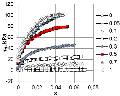
Figure 3a. Dependence of \tau_N on compressive deformation of MRM (mode 4) at different magnetic field induction.
